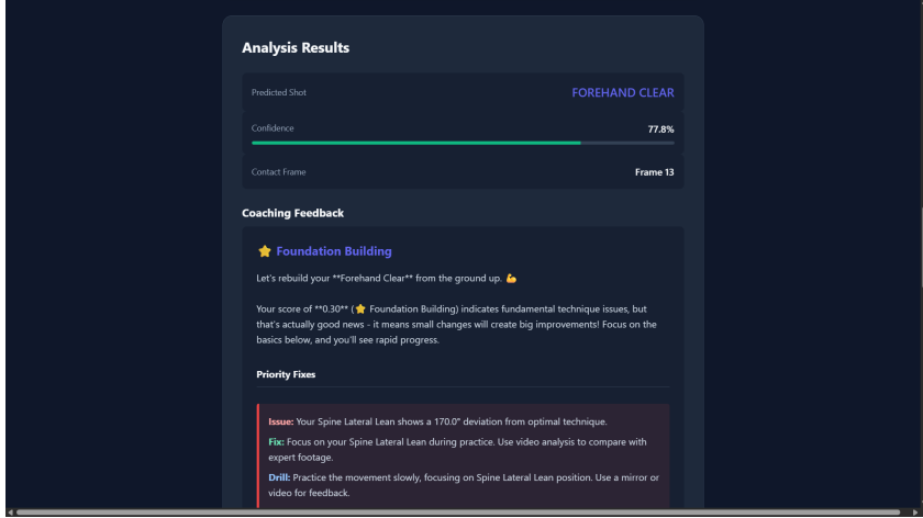
Fig. 10 Smashifix Analysis Results panel showing stroke classification (Forehand Clear, 77.8% confidence), contact frame identification, and KSI-driven coaching feedback with prioritized biomechanical corrections and drill recommendations.
